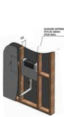
Slimline Dual Flush Concealed Cistern Compatible with WCS002 & Mini Cube units. (See Furniture section) CODE SLCC01N PRICE £71.99
