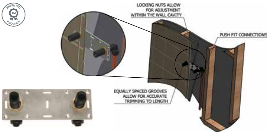
Bar Valve Fixing Plate CODE BVFP01 PRICE £29.99
